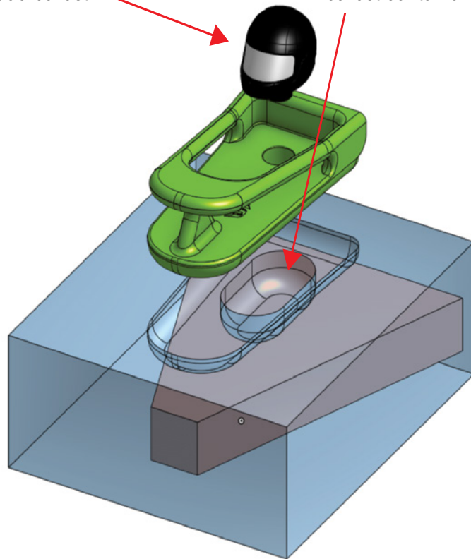
Halo Pocket & Ballast Container Drawing
