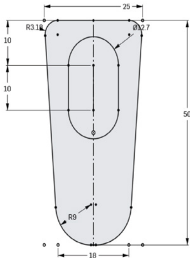
Halo Pocket & Ballast Container Drawing
